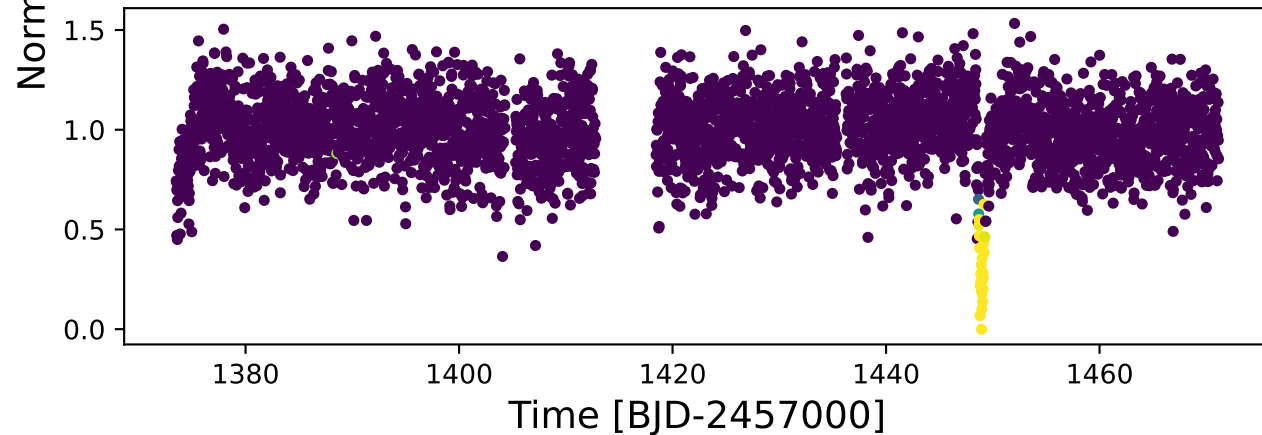
Single Model Predictions - KIC 8027456
