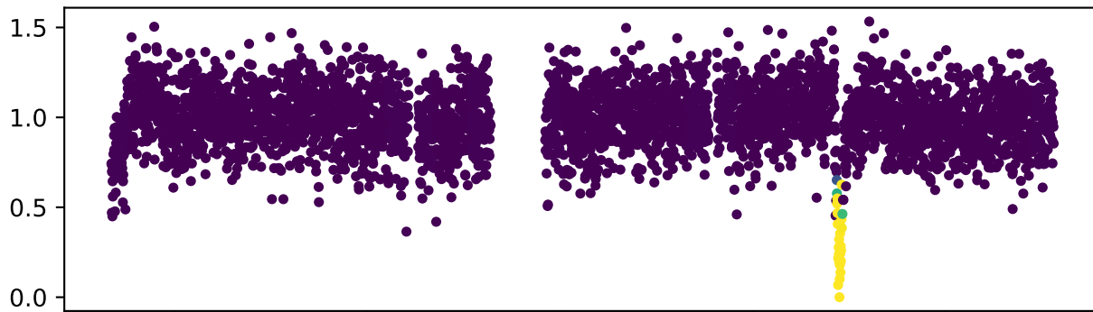
Single Model Predictions - KIC 8027456
